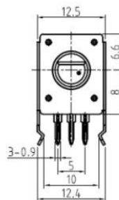
P.C.B.MOUNTING DETAIL
