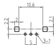
P.C.B.MOUNTING DETAIL
