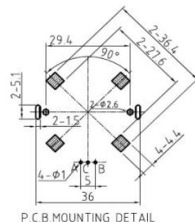
P.C.B. MOUNTING DETAIL
