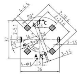
P.C.B MOUNTING DETAIL
