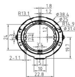
P.C.B MOUNTING DETAIL
