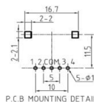
P.C.B MOUNTING DETAIL
