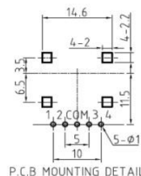
P.C.B MOUNTING DETAIL
