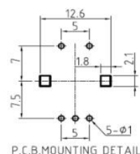
P.C.B.MOUNTING DETAIL
