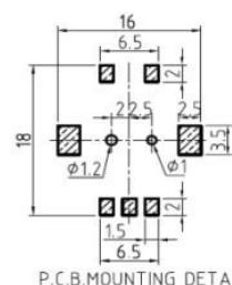
P.C.B. MOUNTING DETAIL
