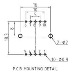
P.C.B MOUNTING DETAIL
