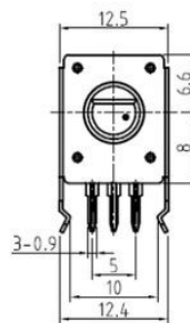
P.C.B.MOUNTING DETAIL
