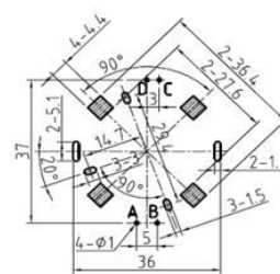
P.C.B. MOUNTING DETAIL
