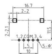
P.C.B. MOUNTING DETAIL
