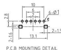
P.C.B MOUNTING DETAIL
