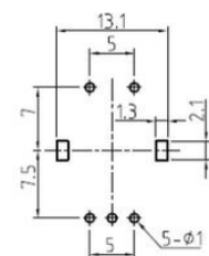
P.C.B. MOUNTING DETAIL
