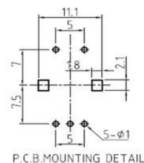
P.C.B.MOUNTING DETAIL
