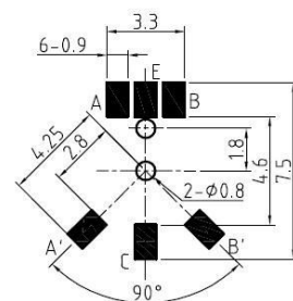
P.C.B.MOUNTING DETAIL
