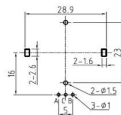
P.C.B. MOUNTING DETAIL
